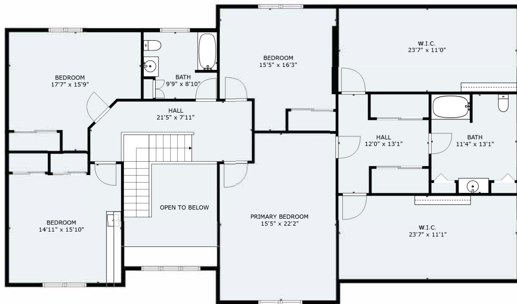
FLOOR 2
