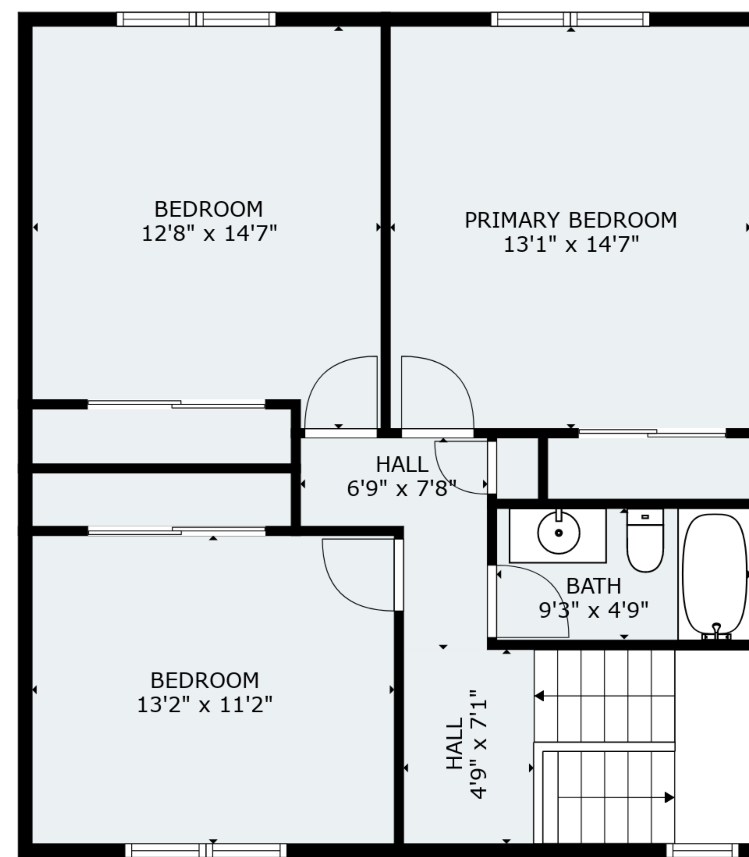
FLOOR 3
