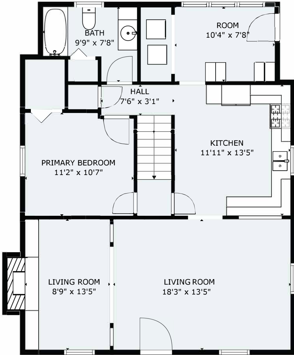
FLOOR 1
