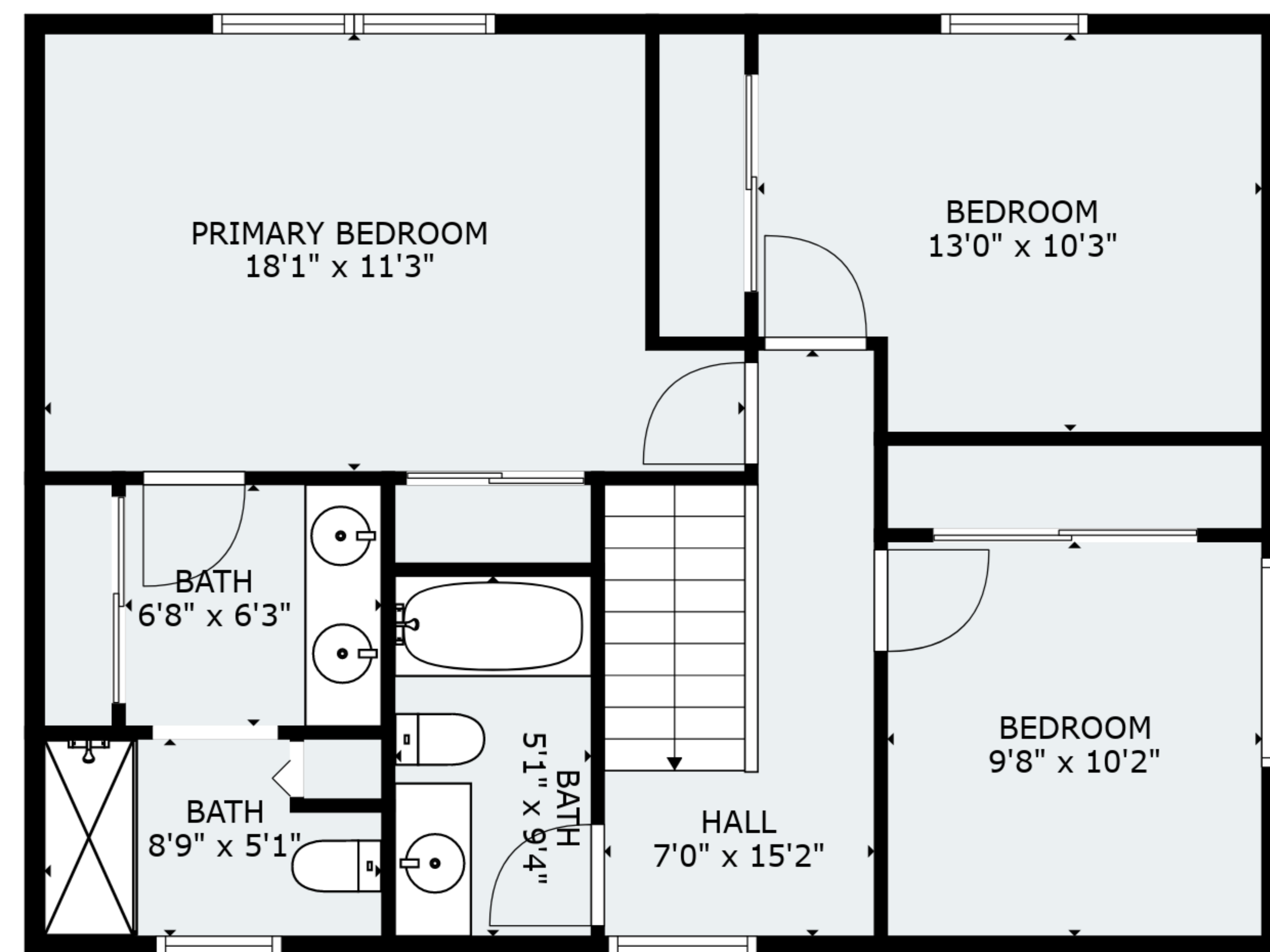
FLOOR 3
