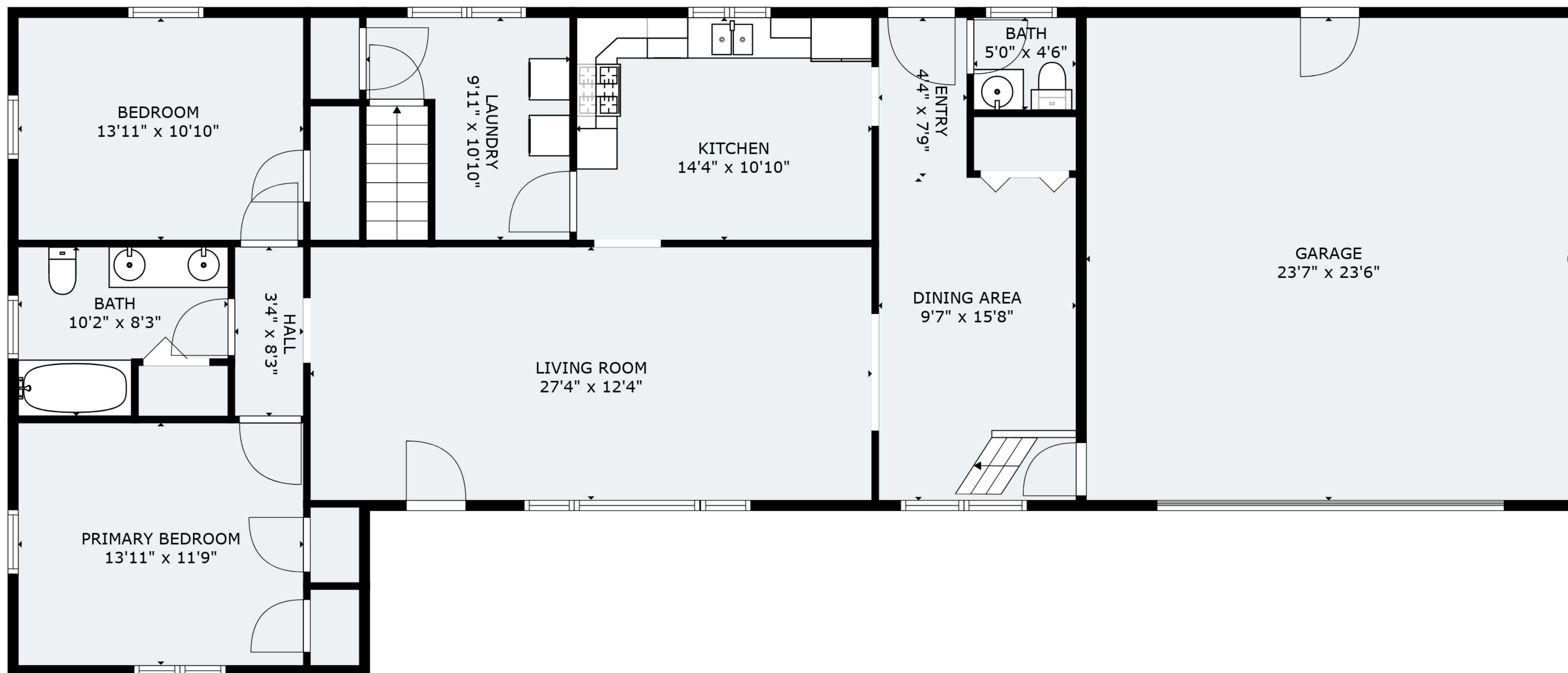
FLOOR 2
