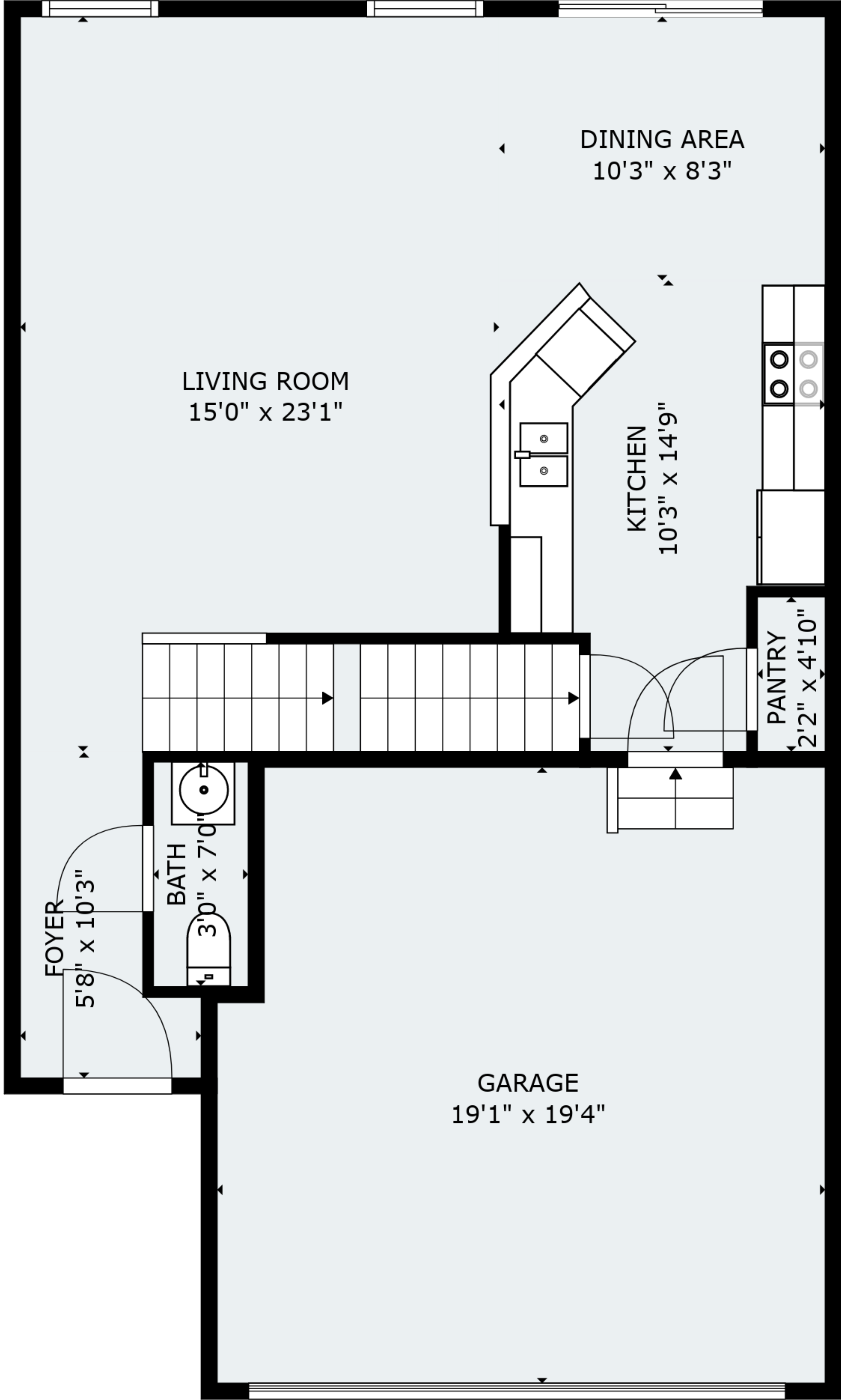
FLOOR 2
